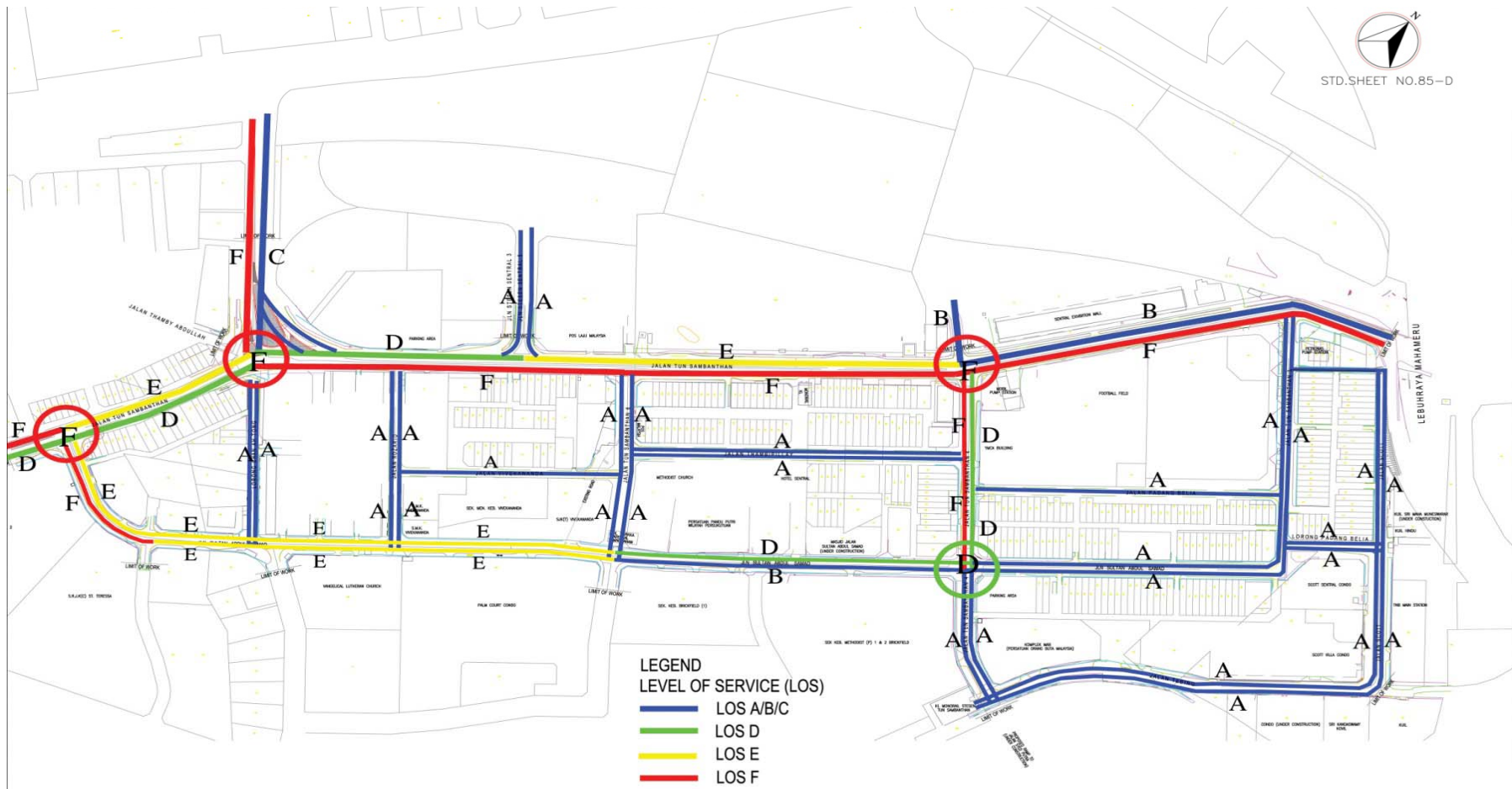
PROPOSED TRAFFIC DISPERSAL SCHEME FOR BRICKFIELDS AREA AND KL SENTRAL STATION AND ITS VICINITY (PACKAGE 3)
